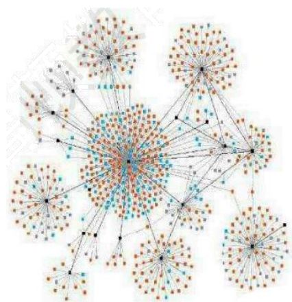
Divisive clustering
